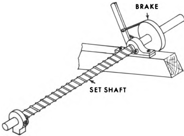
Figure 8-17. Spring-actuated receder.
